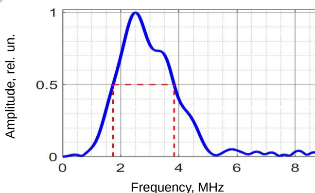
Amplitude frequency response
